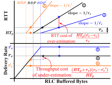
Fig. 6— Cost of errors. L4Span marks the packet using the estimated egress rate and a queuing delay threshold \tau_s . Stars (★) mark the ideal operation points with the estimated egress rate.
