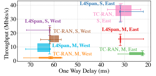
(b) Performance of CUBIC under L4Span and TC-RAN
