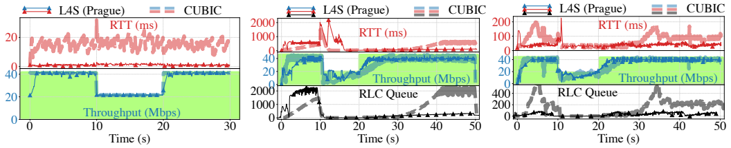
(a) CUBIC and L4S in a wired network. (b) CUBIC and L4S in a 5G network. (c) CUBIC and L4S in 5G + L4Span.
